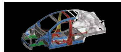
Collision-Resistant Body
